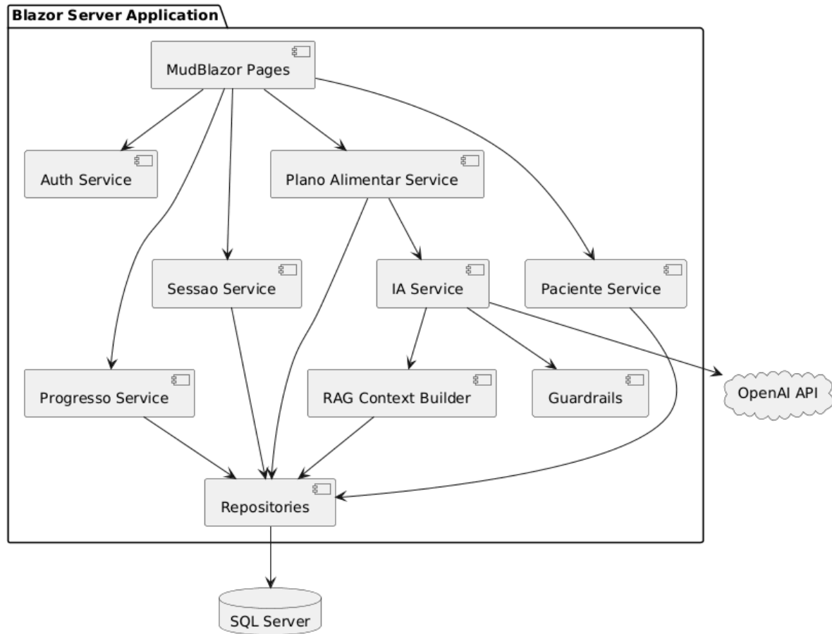
C4 - Component Diagram - NutriIA
